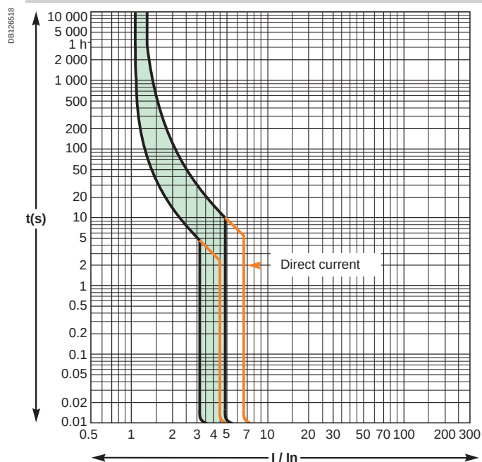
Curve B
