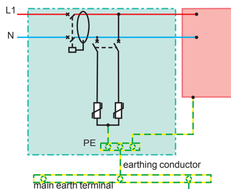
Connection example.
