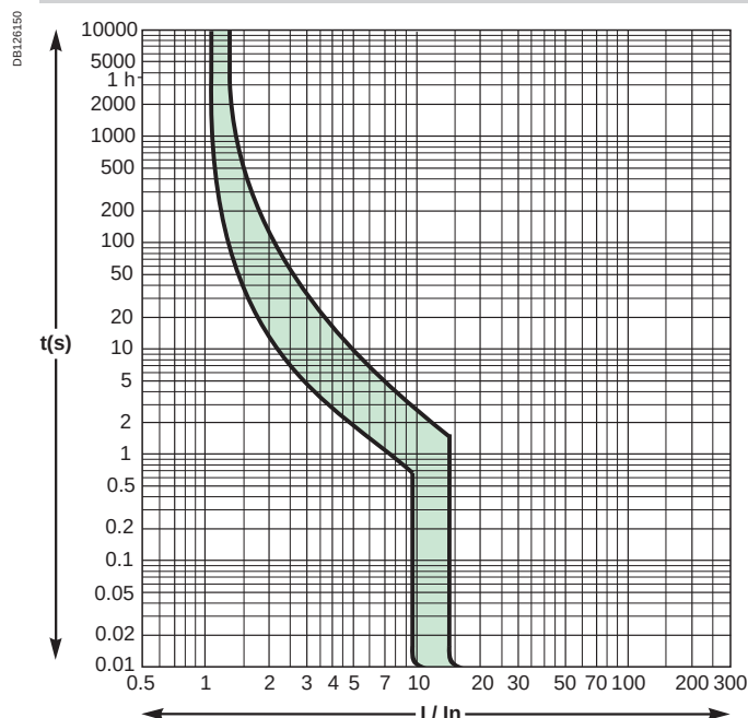
Curve D
