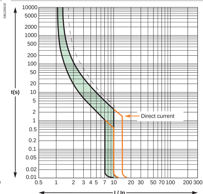
Curve C
