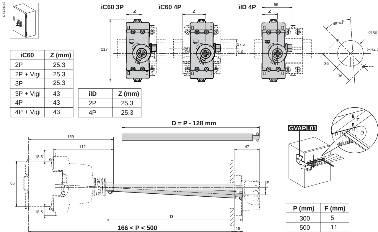
Rotary handle: front mounted control
