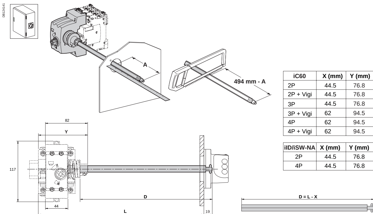
Rotary handle: side mounted control
